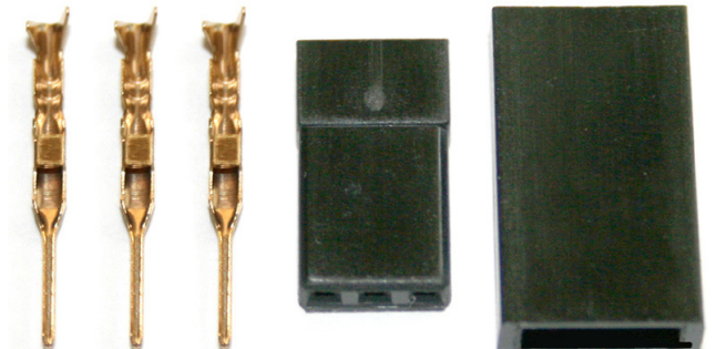
HRC9202B UNI female plug (20 pcs)
